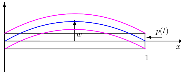
FIGURE 1. The beam; w is the displacement of the central axis.
